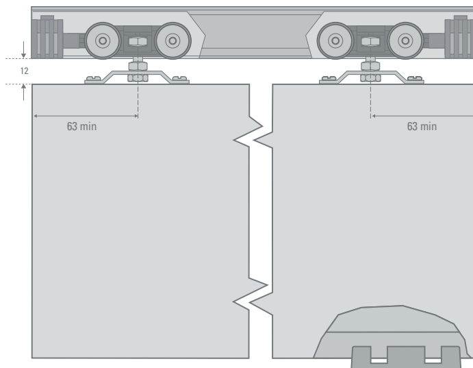
Vista Frontal
